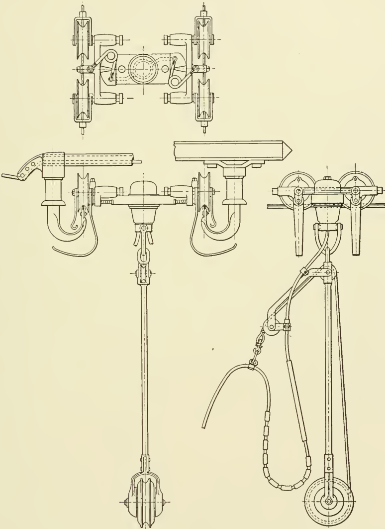
Fig. 7. Plan and Front and Side Elevation of Mercedes-Stoll Current Collector
